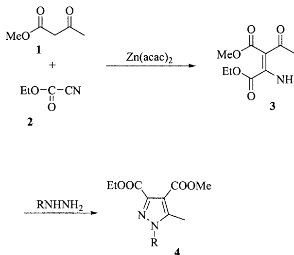
Scheme 1. Synthesis of pyrazoledicarboxylic acid derivatives.
