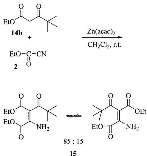
Scheme 5. Synthesis of compound 15 .
