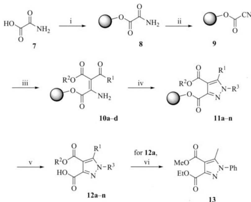
Scheme 3. Solid-phase synthesis of pyrazoledicarboxylic acid derivatives 12 . See Table 1 for R^1 , R^2 and R^3 . Reagents and conditions: i: 2,6-dichlorobenzoyl chloride, pyridine, Wang resin ( 5 ), DMF, 0 °C; ii: TFAA, pyridine, dichloromethane, 0 °C; iii: R^1\text{COCH}_2\text{COOR}^2 ( 1 or 14a–c ), \text{Zn}(\text{acac})_2 , \text{CH}_2\text{Cl}_2 , room temp.; iv: R^3\text{NHNH}_2 , \text{CH}_2\text{Cl}_2 , room temp.; v: TFA/ \text{CH}_2\text{Cl}_2 (3:1 vol/vol), room temp.; vi: \text{SOCl}_2 followed by EtOH, 0 °C, then reflux.
