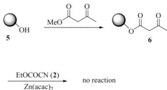
Scheme 2. First approach to the synthesis of resin-bound enamino keto diesters of type 3 .
